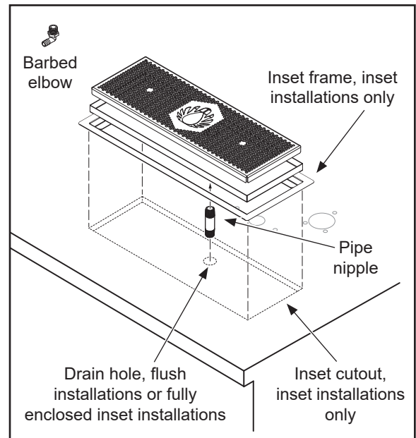
Figure 5 - Drip Tray Installation
