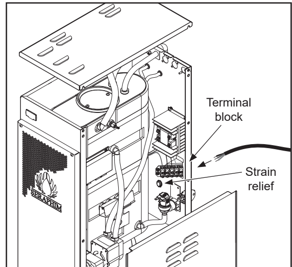
Figure 1 - Power Cord Connection
