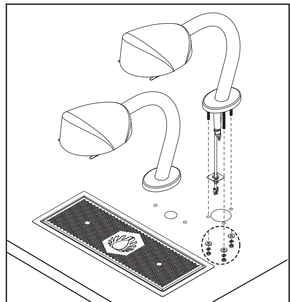
Figure 6 - Brew Head Installation
