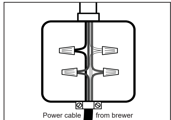
Figure 18 - Junction Box Connection
