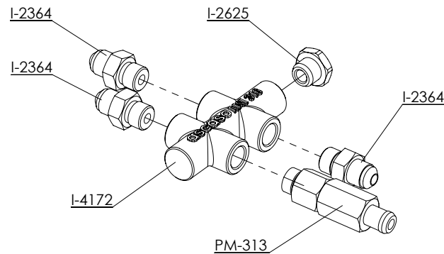
PM-389 (Coffee circuit water distributor Barista T 2Gr)
